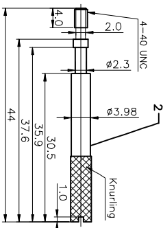
SCREW-1
