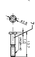
Short BOLT
